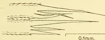
TEXT-FIG. 6.— Baccalaurus japonicus Broch. Rami of caudal fork, showing arrangement of terminal spines.
